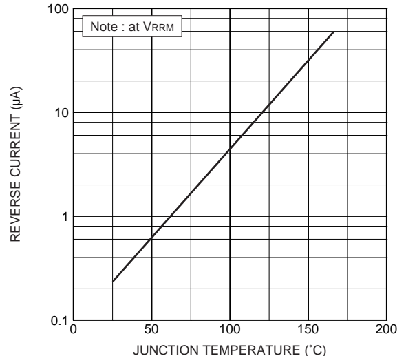
Typ. Reverse current vs. junction temperature
